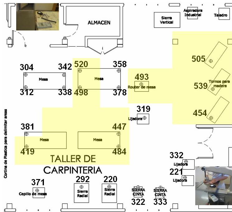
Figure 1. Location of adequate lighting in each of the workstations
