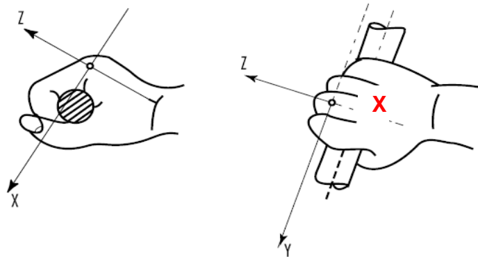
Figure 2: Coordinates system for the measuring of the vibrations transmitted to the hands.
