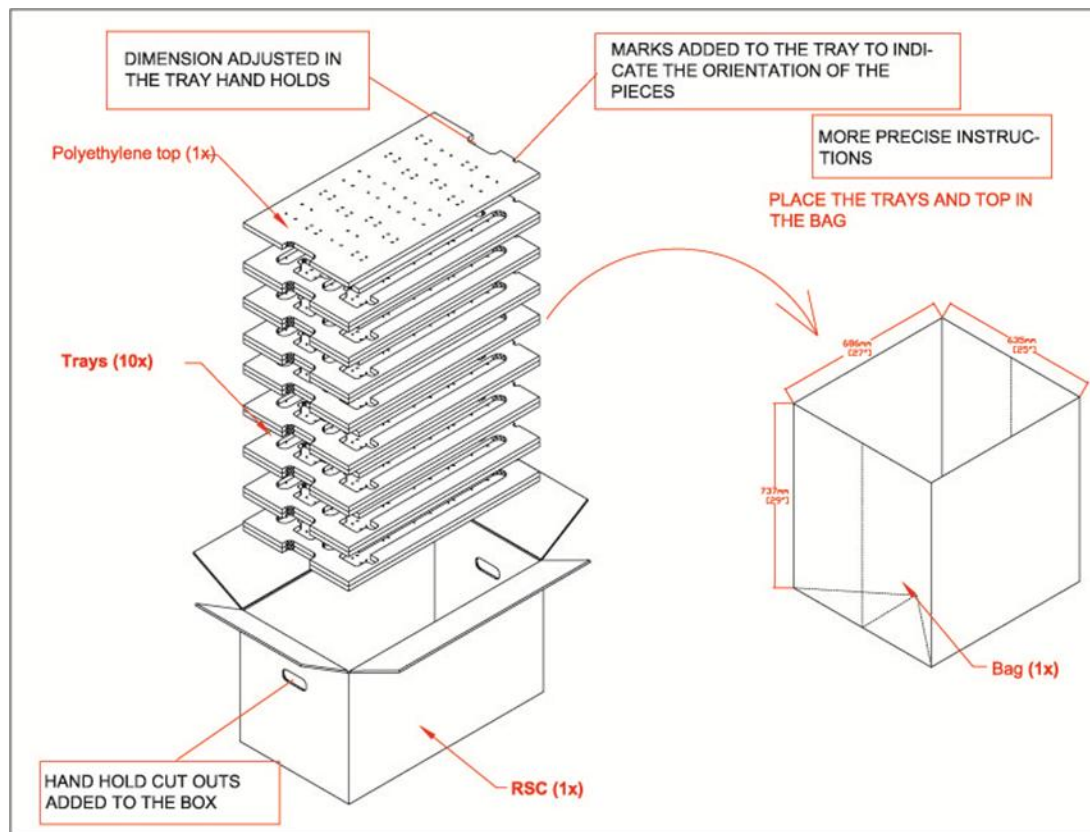
Figure 1. Proposal of containment system.
